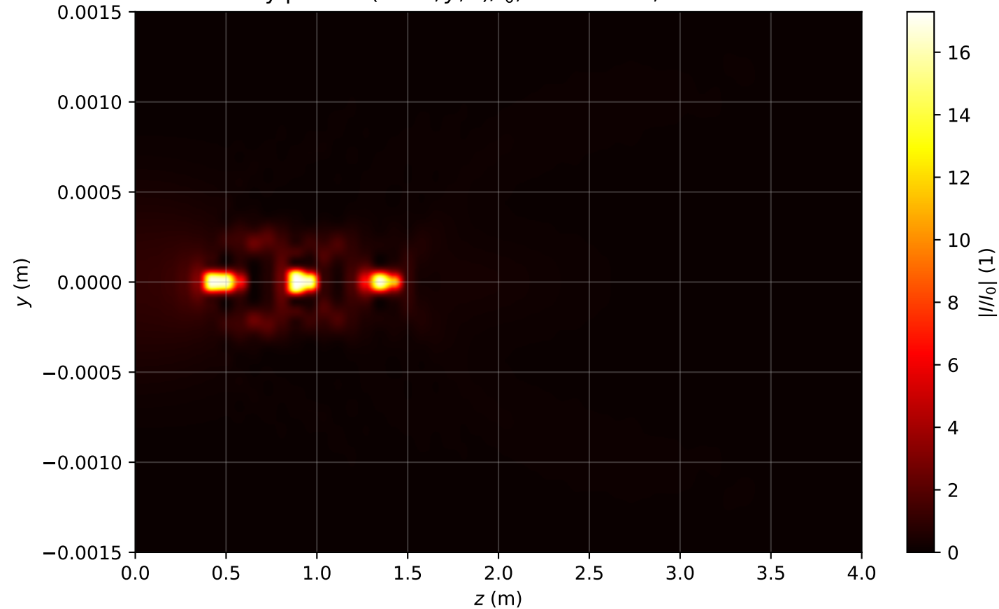
Intensity profile I(x=0, y, z)/I_0 , P_{in}=6.5P_{cr} , artificial time
